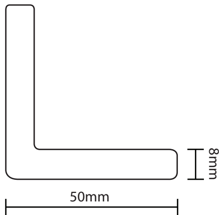
Profile View
